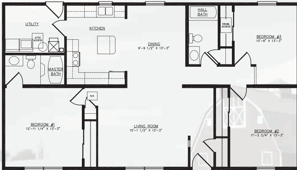
CRAWLSPACE PLAN
